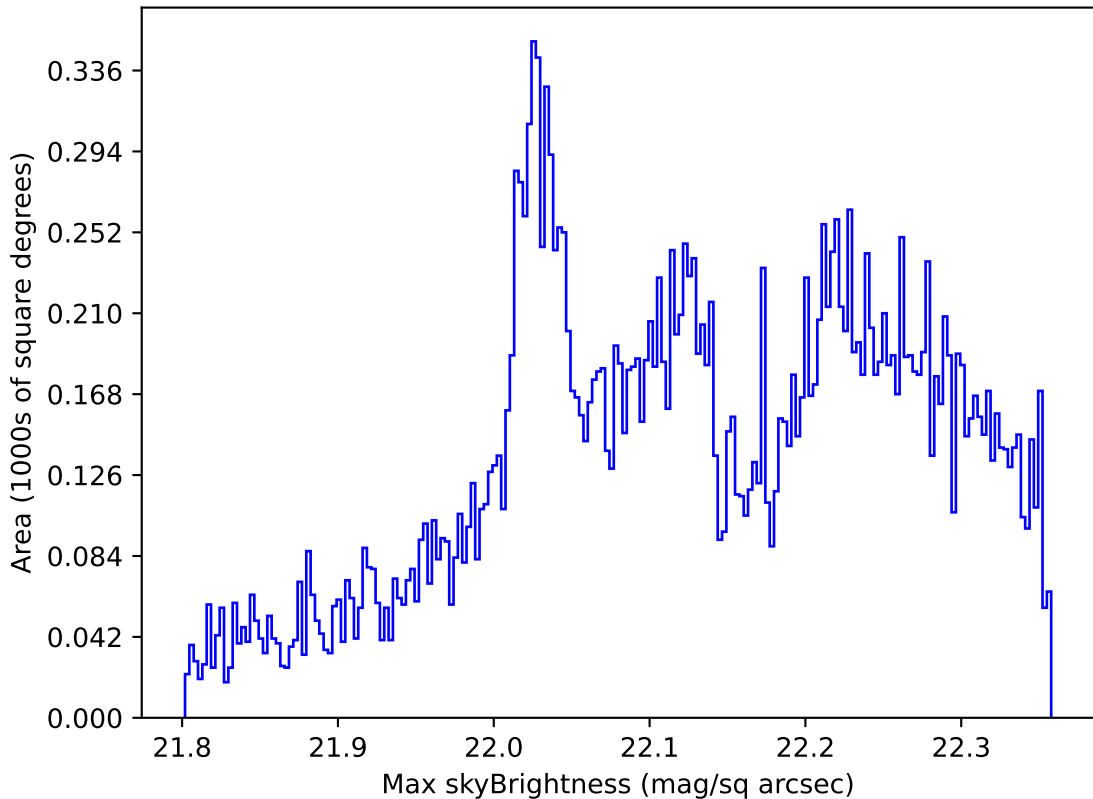
too_elab_r16_d3_griz_v3.4_10yrs All sky g band: Max skyBrightness
