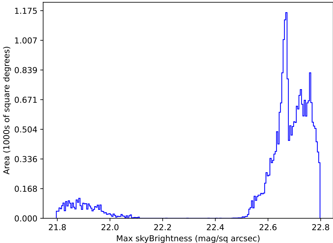
too_elab_r16_d3_griz_v3.4_10yrs All sky all bands: Max skyBrightness
