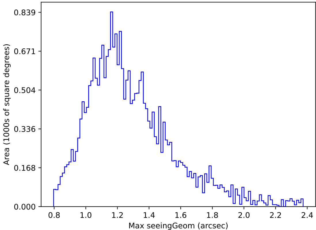
too_elab_r16_d3_griz_v3.4_10yrs Yr 1 z band: Max seeingGeom
