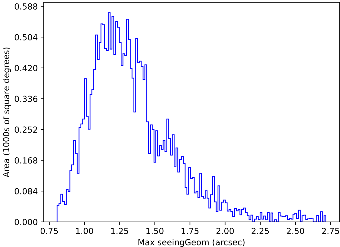
too_elab_r16_d3_griz_v3.4_10yrs Yr 1 u band: Max seeingGeom
