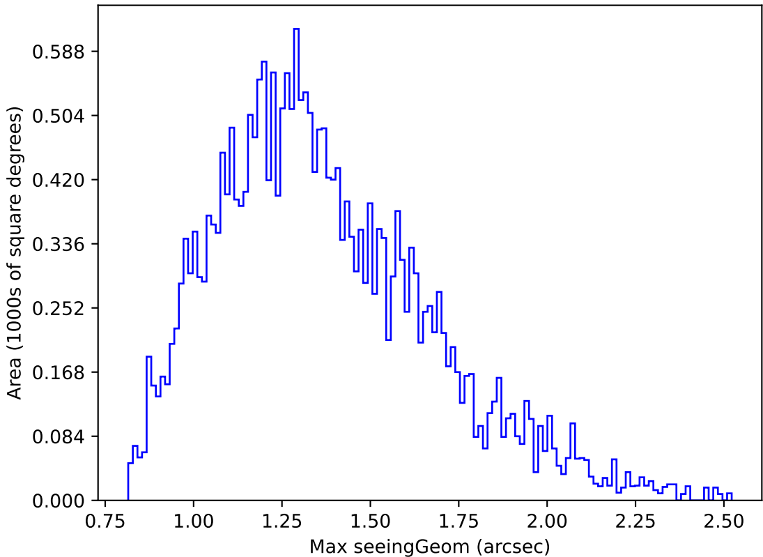
too_elab_r16_d3_griz_v3.4_10yrs Yr 1 r band: Max seeingGeom
