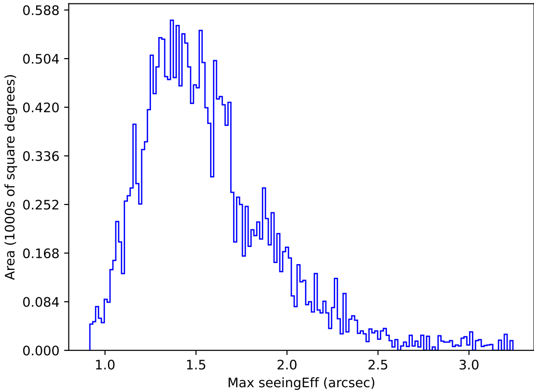
too_elab_r16_d3_griz_v3.4_10yrs Yr 1 u band: Max seeingEff
