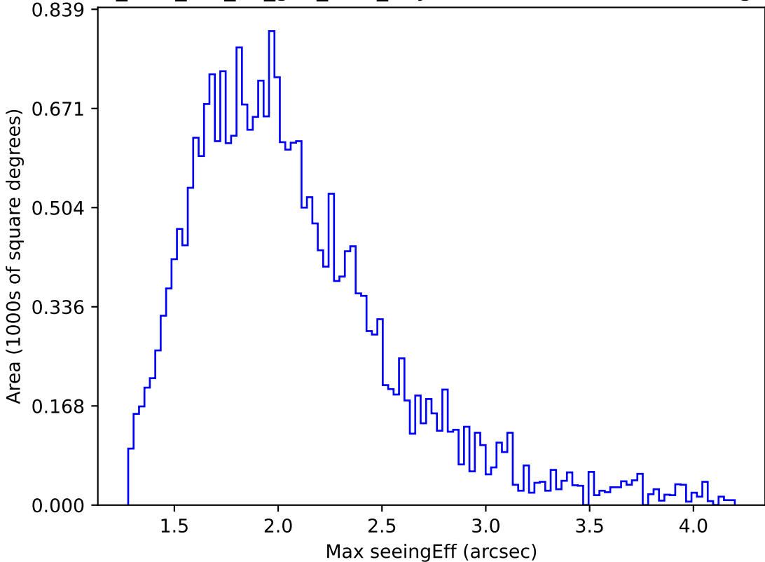
too_elab_r16_d3_griz_v3.4_10yrs Yr 1 all bands: Max seeingEff
