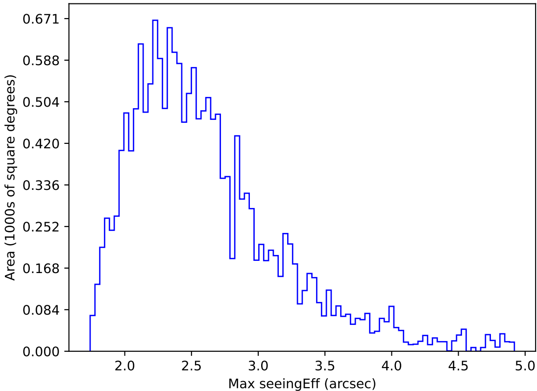
too_elab_r16_d3_griz_v3.4_10yrs WFD z band: Max seeingEff
