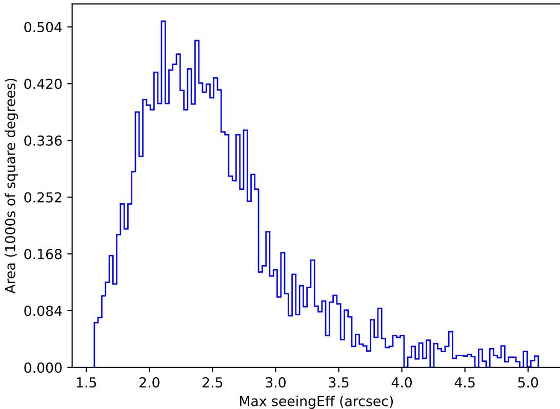
too_elab_r16_d3_griz_v3.4_10yrs WFD y band: Max seeingEff
