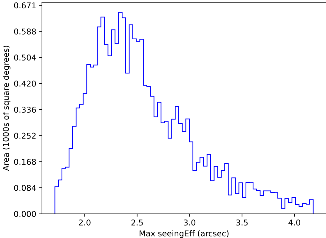
too_elab_r16_d3_griz_v3.4_10yrs WFD u band: Max seeingEff
