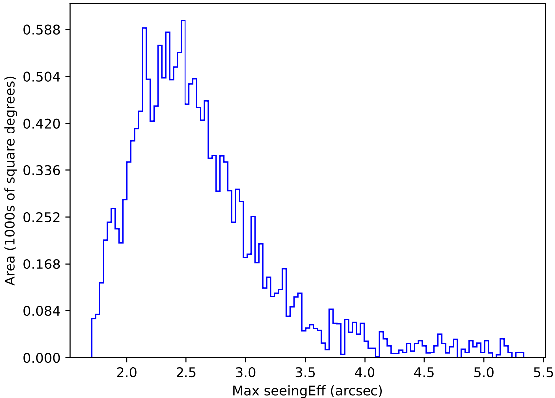
too_elab_r16_d3_griz_v3.4_10yrs WFD i band: Max seeingEff
