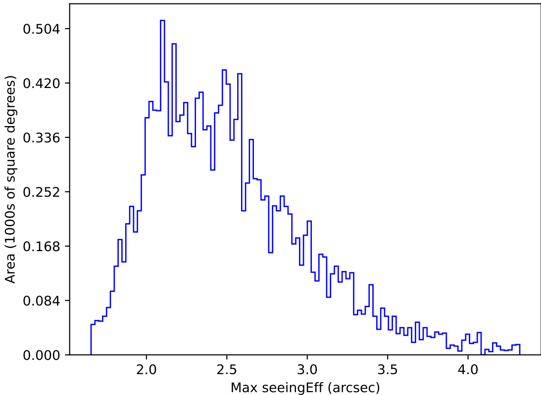
too_elab_r16_d3_griz_v3.4_10yrs WFD g band: Max seeingEff
