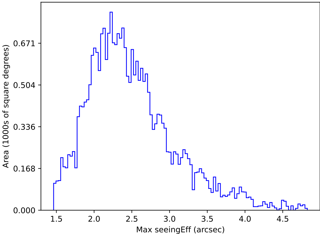
too_elab_r16_d3_griz_v3.4_10yrs All sky z band: Max seeingEff
