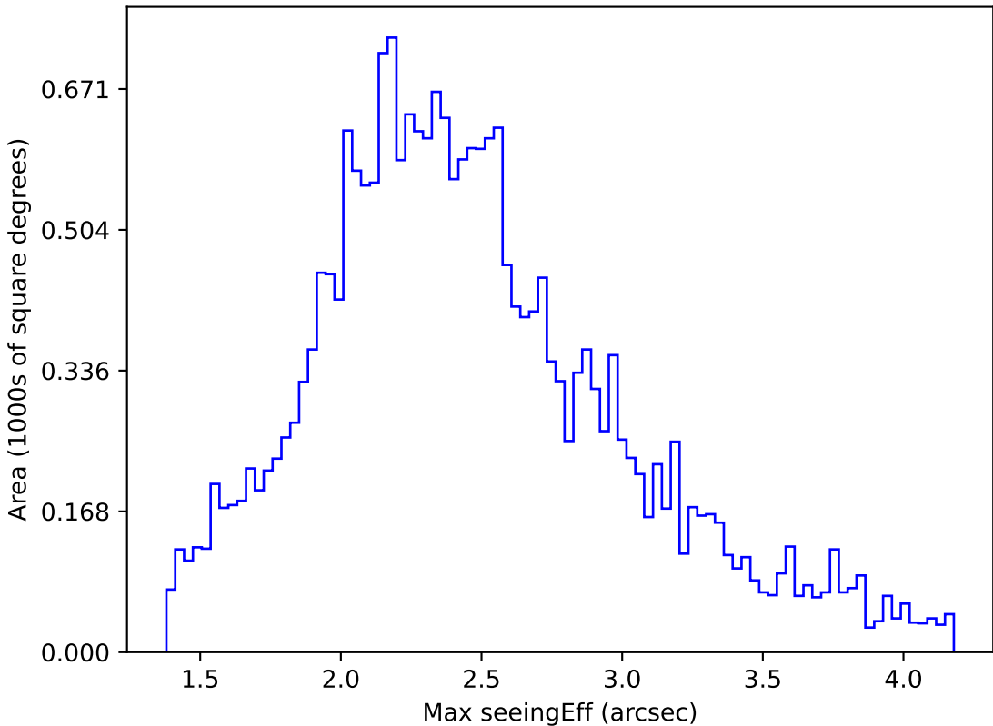
too_elab_r16_d3_griz_v3.4_10yrs All sky u band: Max seeingEff
