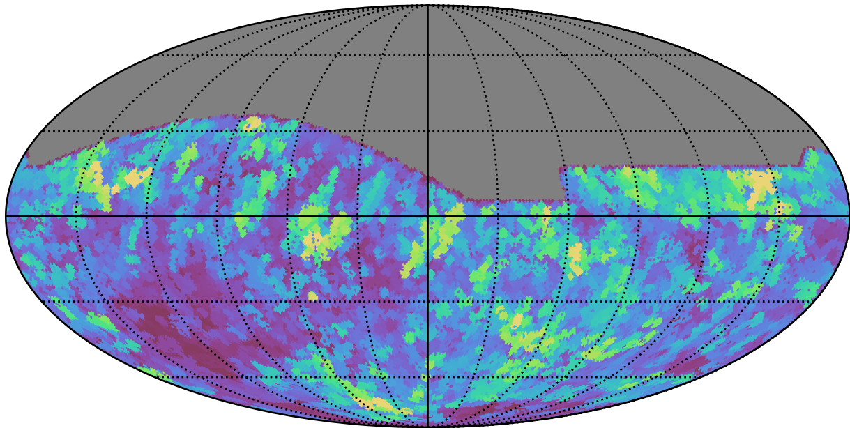
too_elab_r16_d3_griz_v3.4_10yrs All sky r band: Max seeingEff
