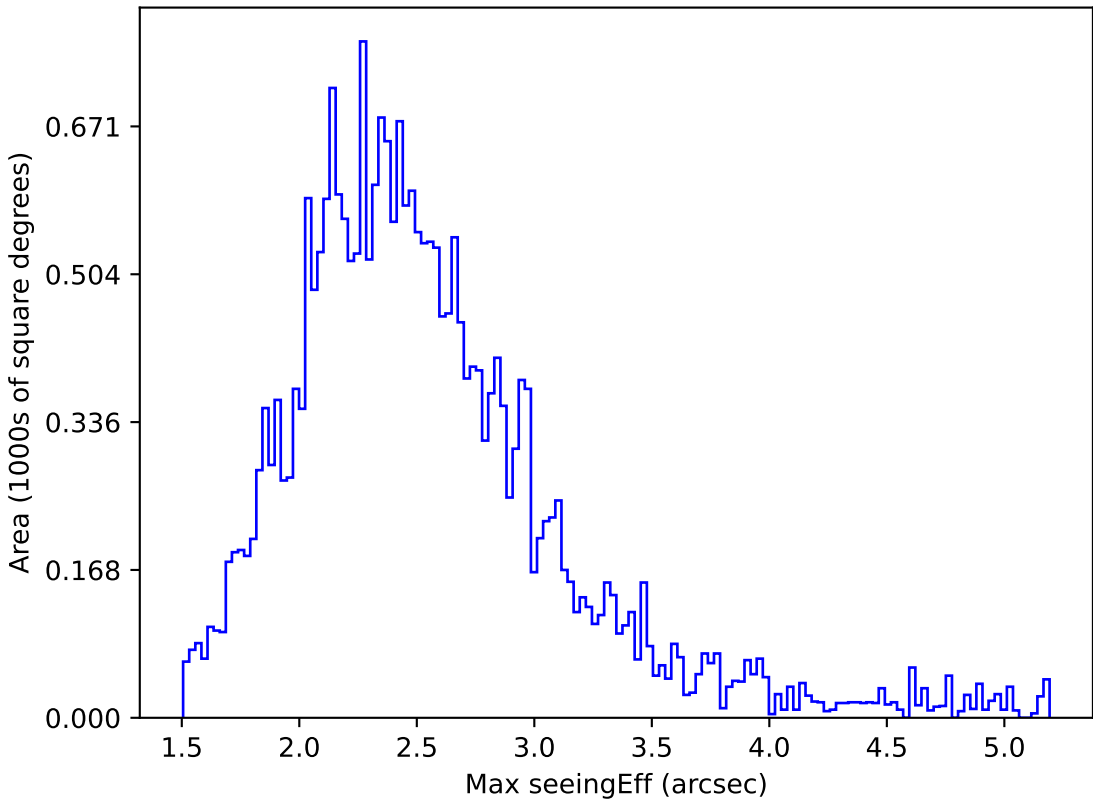
too_elab_r16_d3_griz_v3.4_10yrs All sky i band: Max seeingEff
