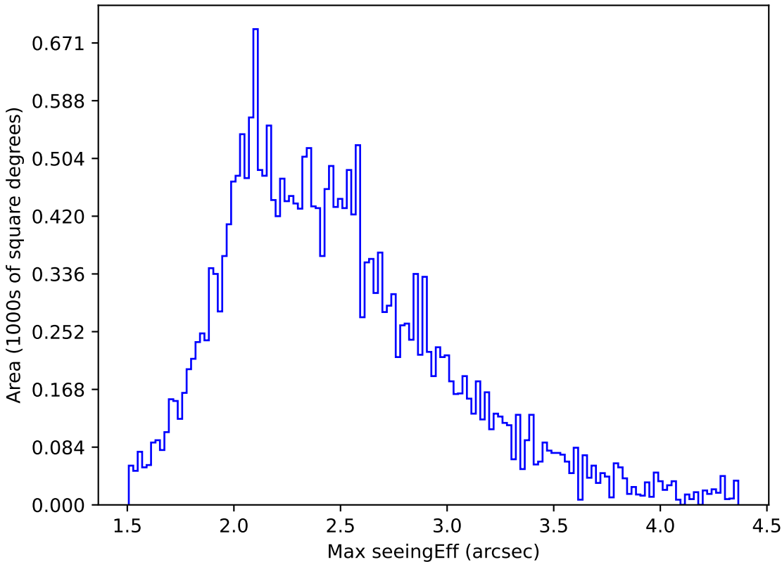
too_elab_r16_d3_griz_v3.4_10yrs All sky g band: Max seeingEff
