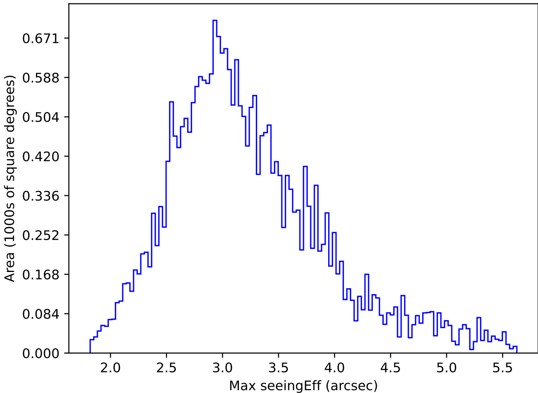
too_elab_r16_d3_griz_v3.4_10yrs All sky all bands: Max seeingEff
