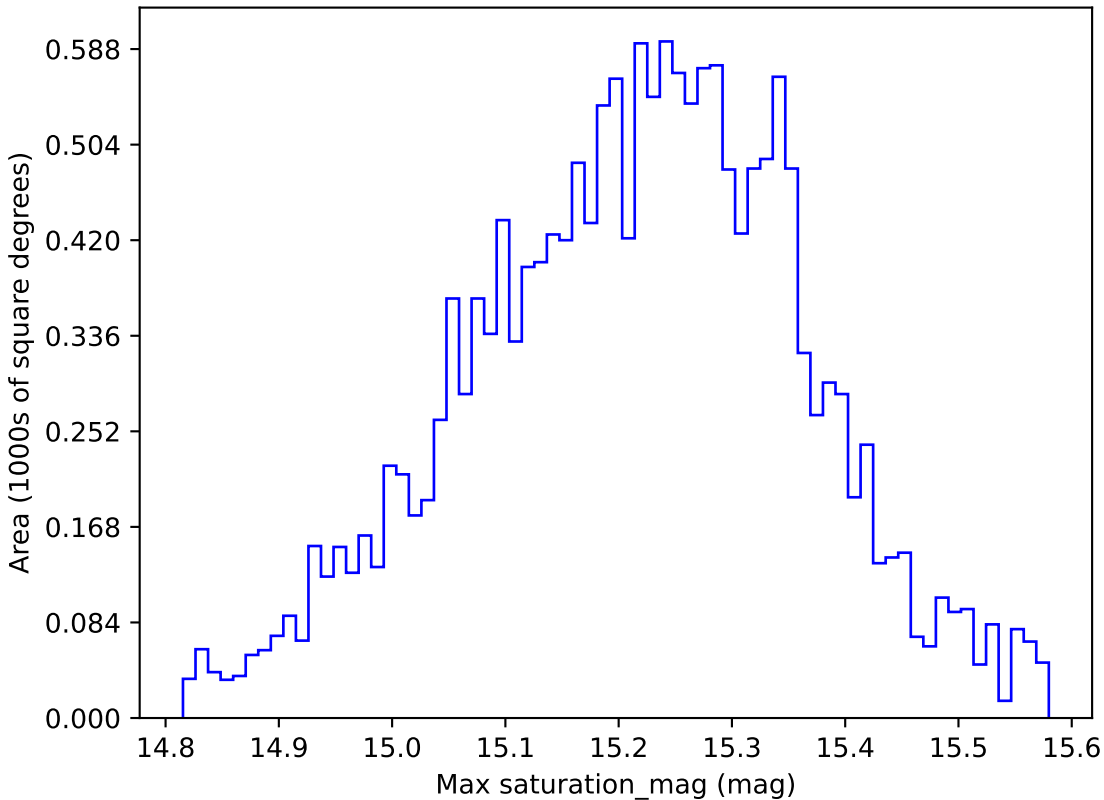
too_elab_r16_d3_griz_v3.4_10yrs WFD z band: Max saturation_mag
