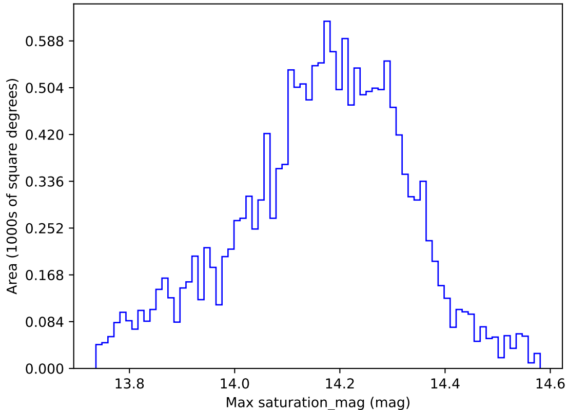
too_elab_r16_d3_griz_v3.4_10yrs WFD y band: Max saturation_mag
