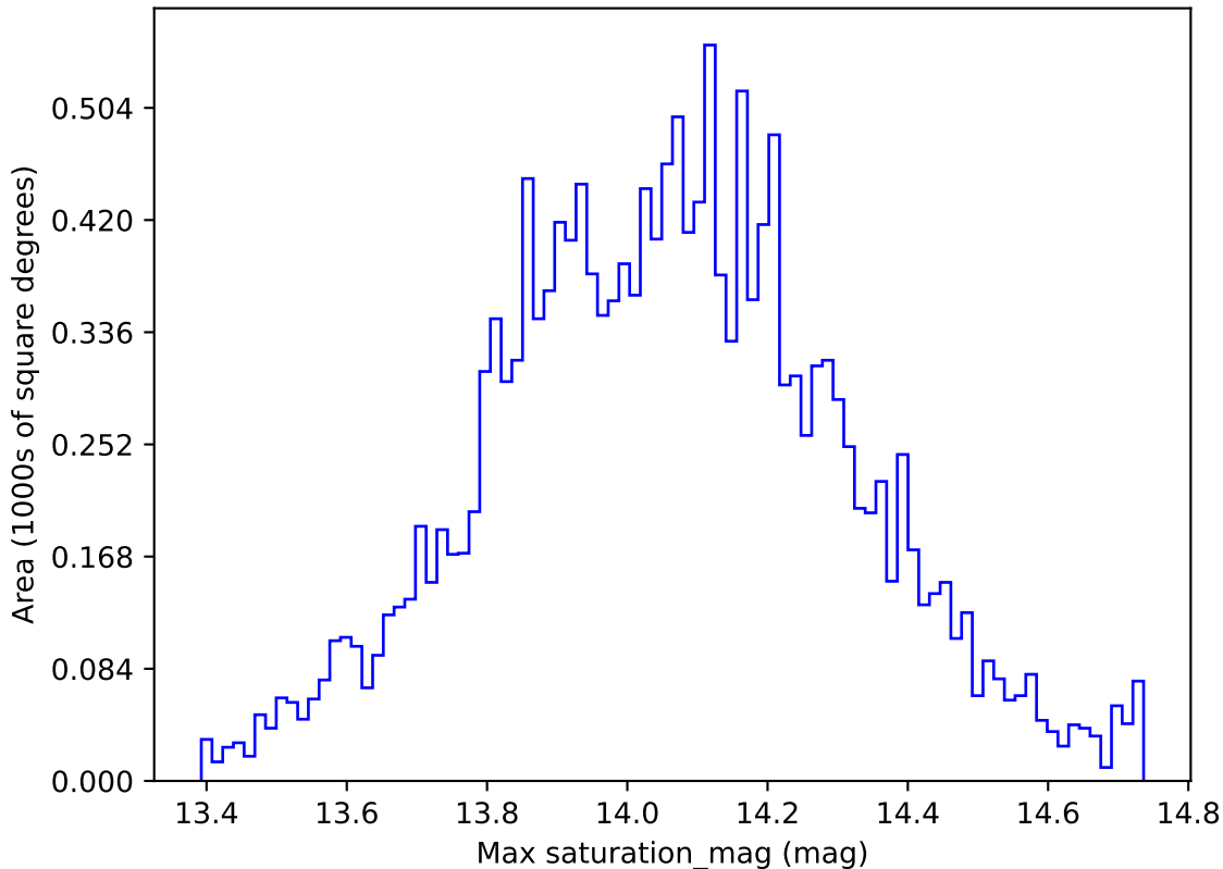
too_elab_r16_d3_griz_v3.4_10yrs WFD u band: Max saturation_mag
