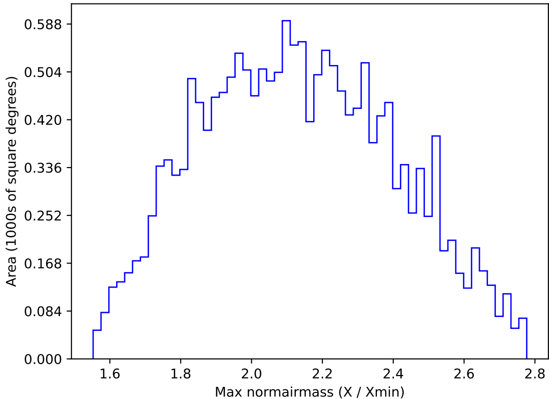
too_elab_r16_d3_griz_v3.4_10yrs WFD y band: Max normairmass
