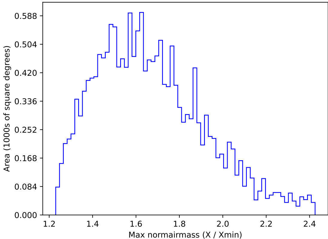
too_elab_r16_d3_griz_v3.4_10yrs WFD u band: Max normairmass
