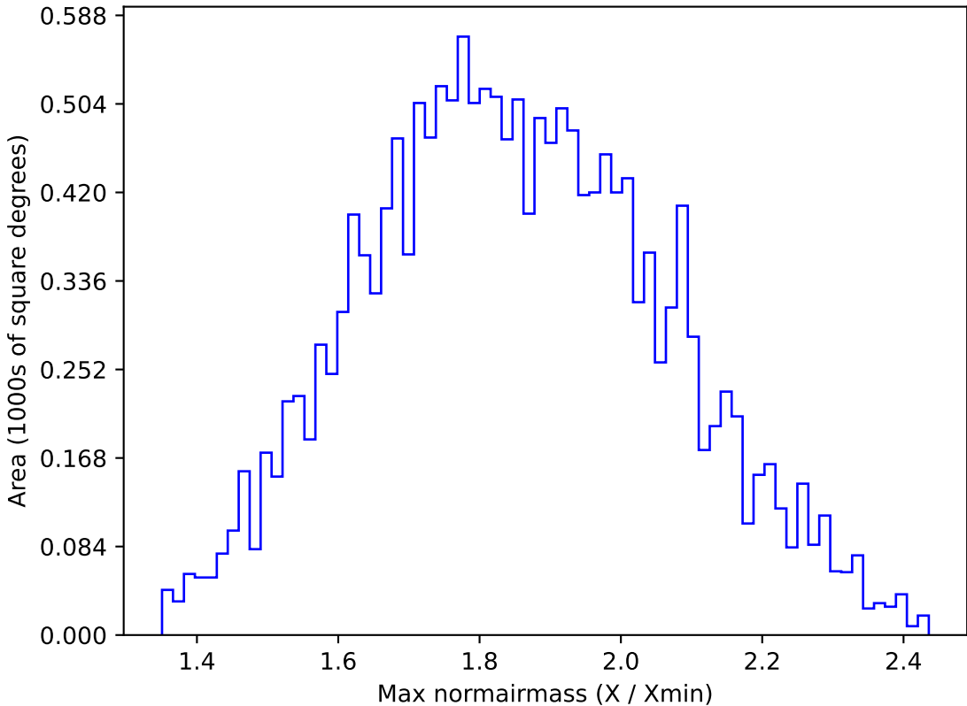
too_elab_r16_d3_griz_v3.4_10yrs WFD g band: Max normairmass
