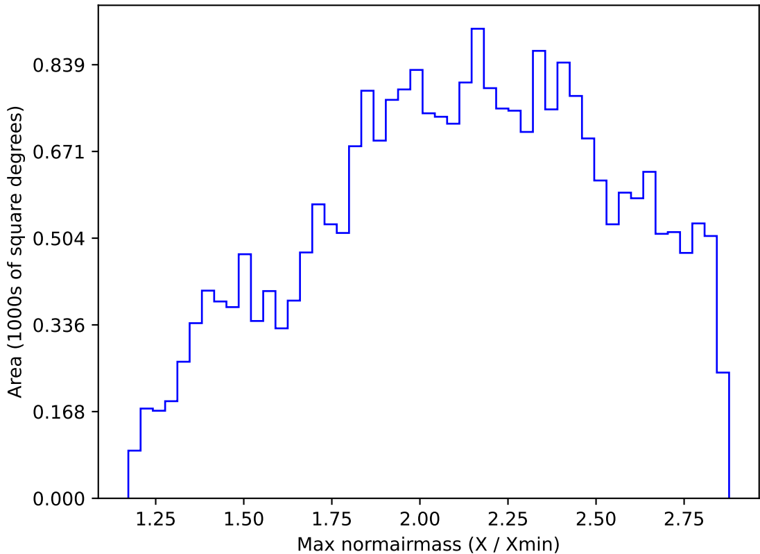
too_elab_r16_d3_griz_v3.4_10yrs All sky z band: Max normairmass
