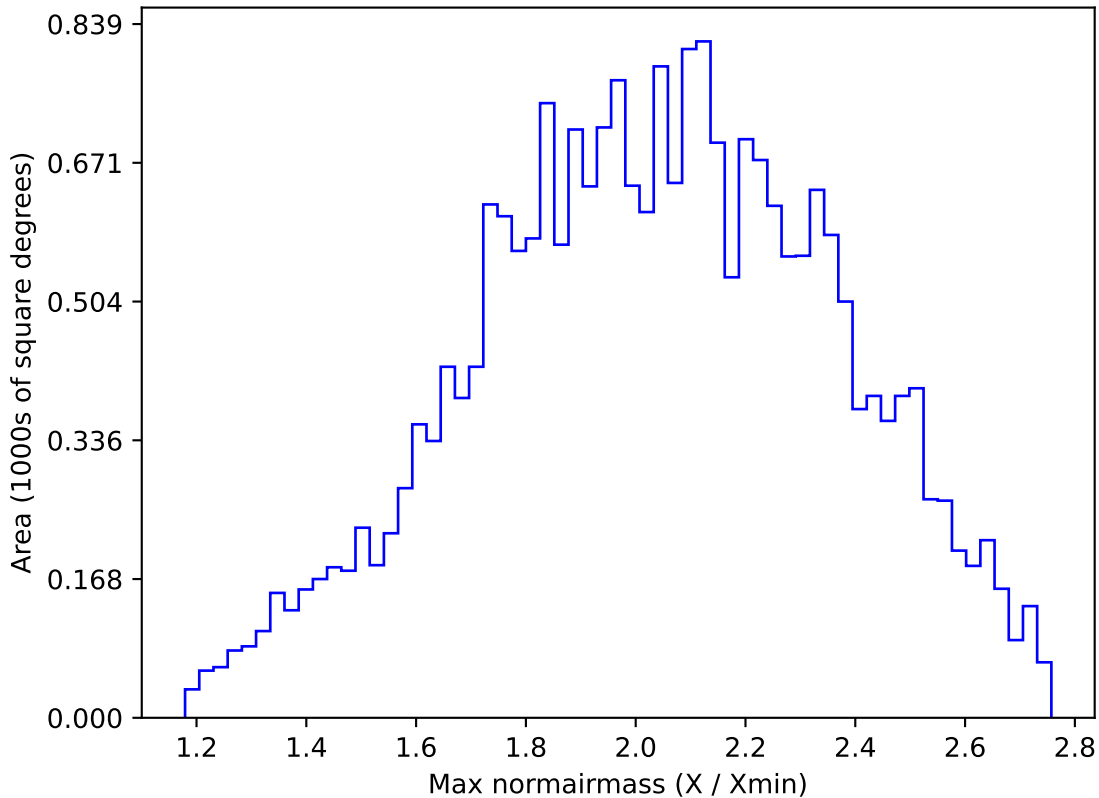
too_elab_r16_d3_griz_v3.4_10yrs All sky y band: Max normairmass
