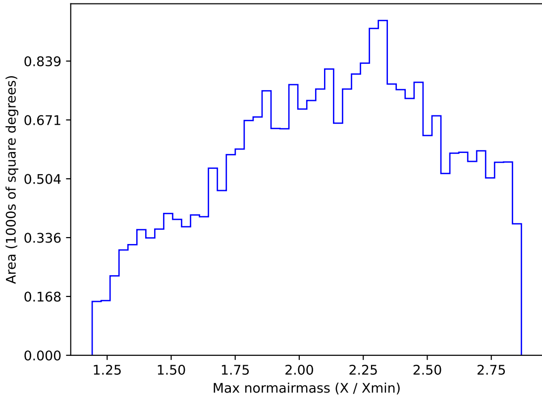
too_elab_r16_d3_griz_v3.4_10yrs All sky i band: Max normairmass
