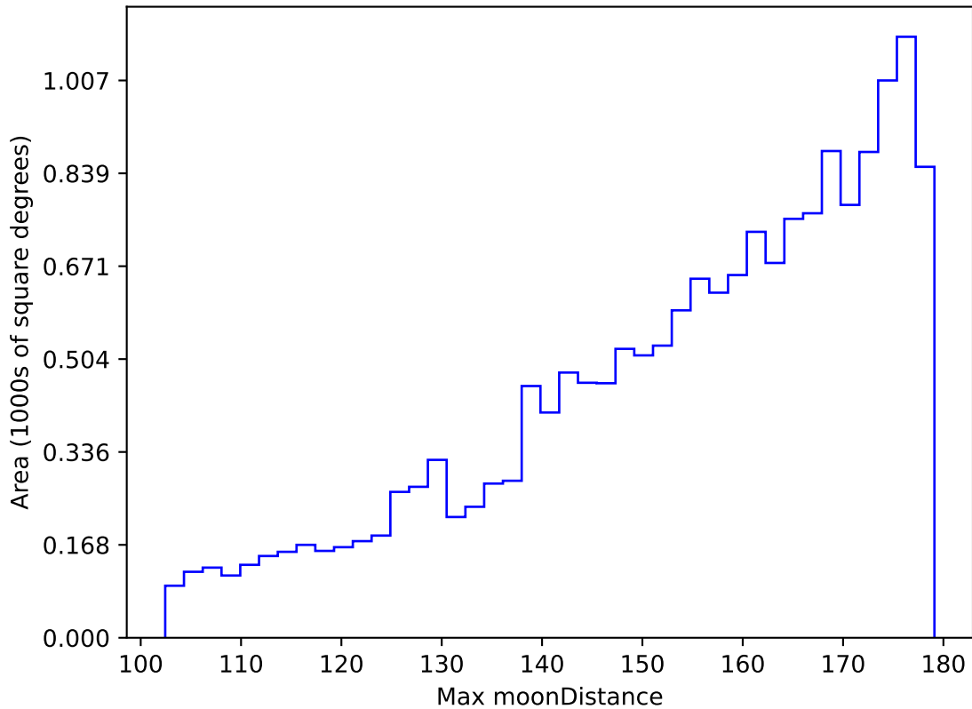
too_elab_r16_d3_griz_v3.4_10yrs WFD z band: Max moonDistance
