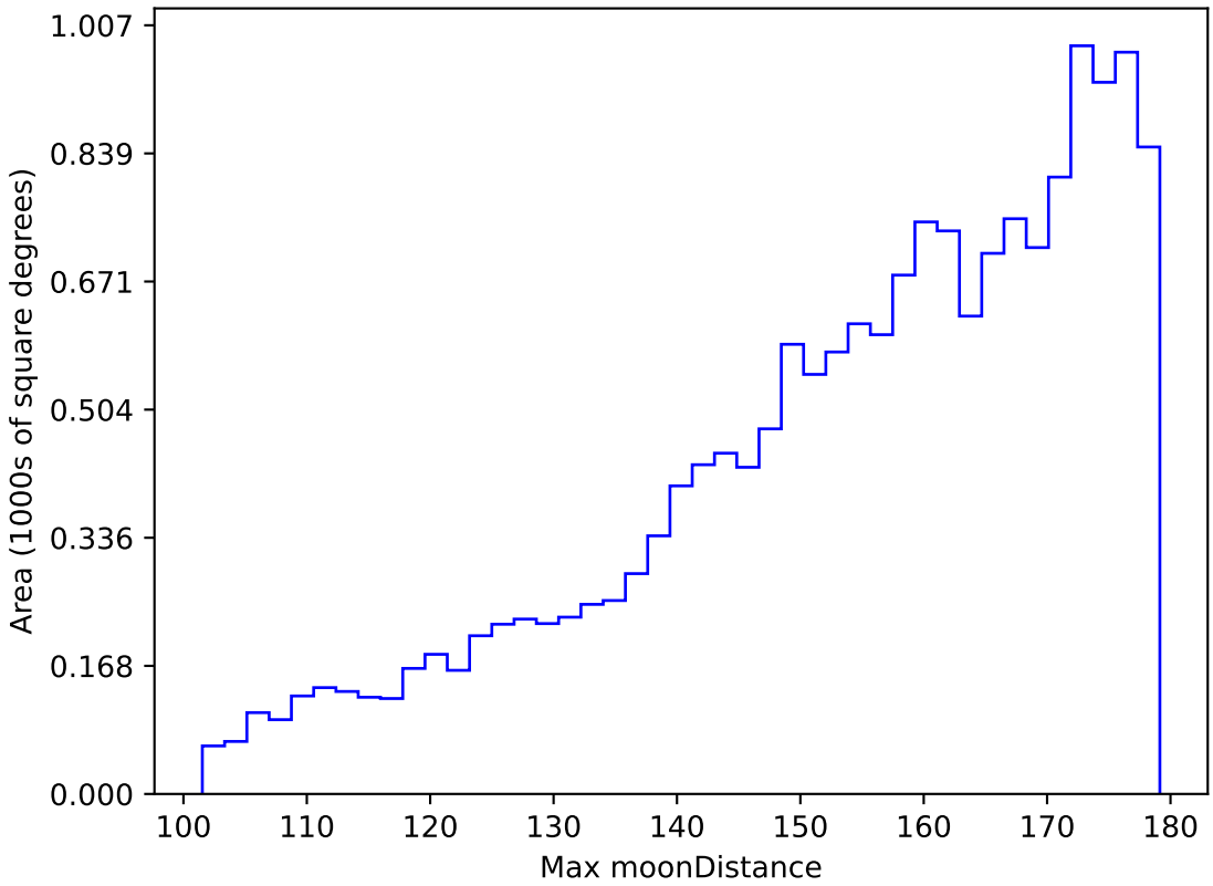
too_elab_r16_d3_griz_v3.4_10yrs WFD u band: Max moonDistance
