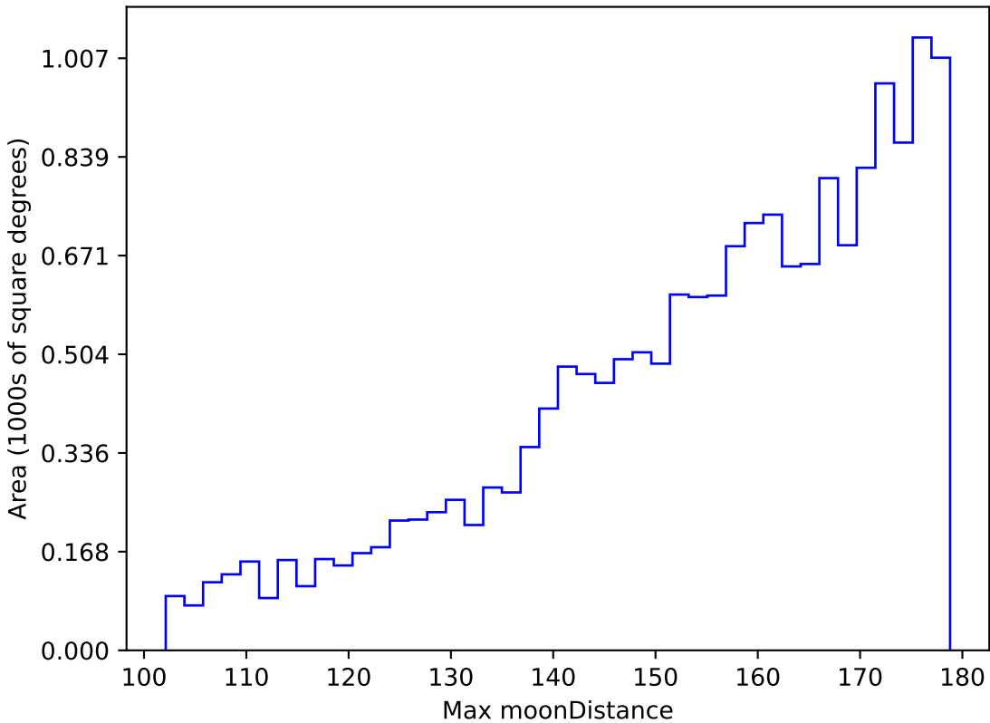
too_elab_r16_d3_griz_v3.4_10yrs WFD g band: Max moonDistance
