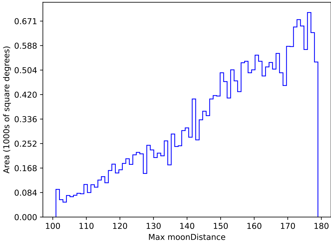
too_elab_r16_d3_griz_v3.4_10yrs All sky u band: Max moonDistance
