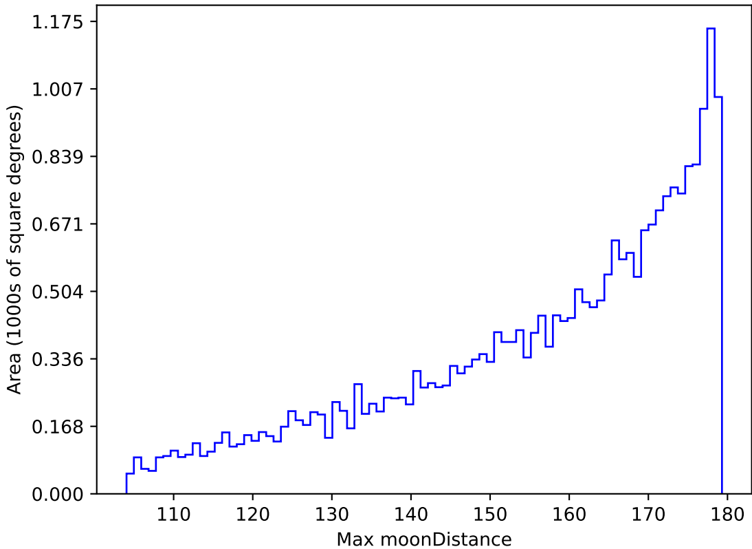
too_elab_r16_d3_griz_v3.4_10yrs All sky r band: Max moonDistance
