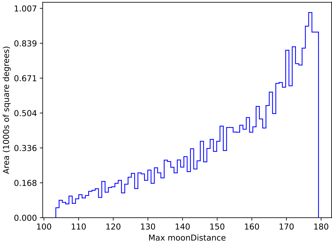
too_elab_r16_d3_griz_v3.4_10yrs All sky i band: Max moonDistance
