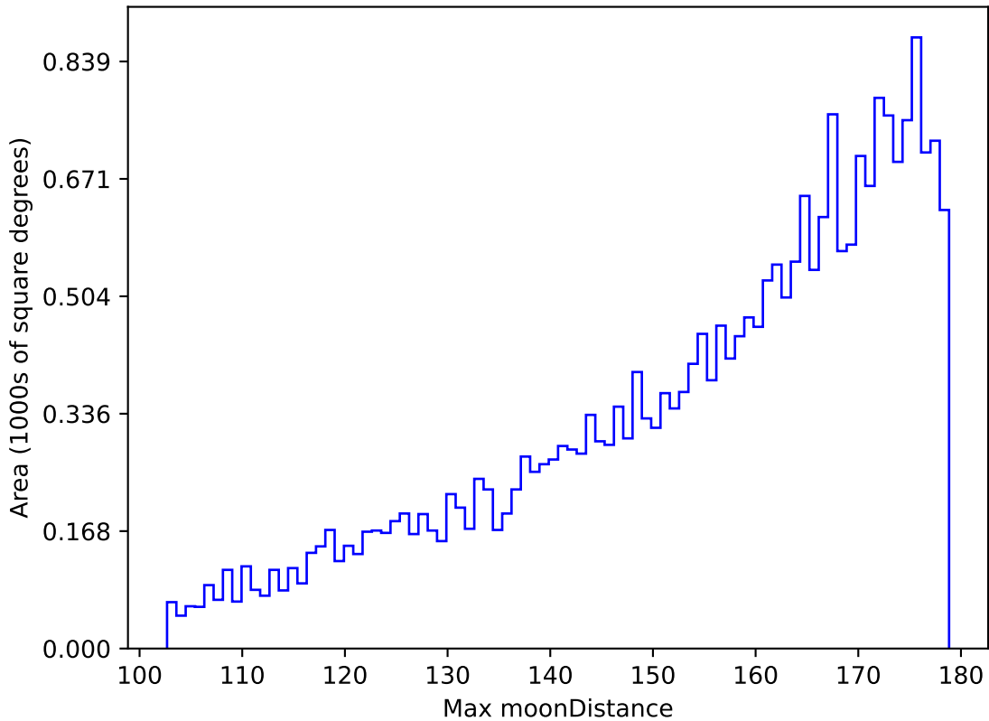
too_elab_r16_d3_griz_v3.4_10yrs All sky g band: Max moonDistance
