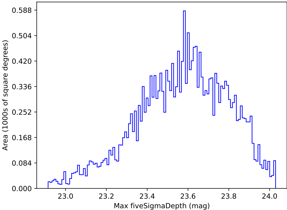
too_elab_r16_d3_griz_v3.4_10yrs Yr 1 u band: Max fiveSigmaDepth
