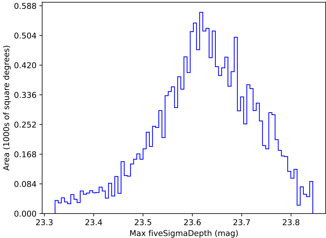
too_elab_r16_d3_griz_v3.4_10yrs WFD z band: Max fiveSigmaDepth
