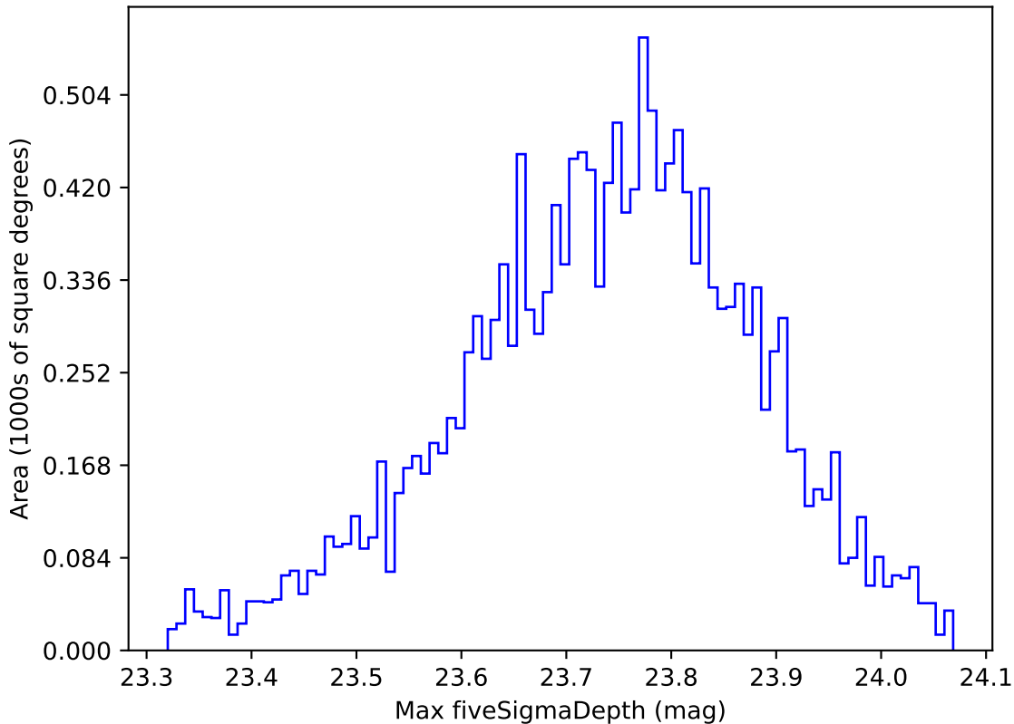
too_elab_r16_d3_griz_v3.4_10yrs WFD u band: Max fiveSigmaDepth
