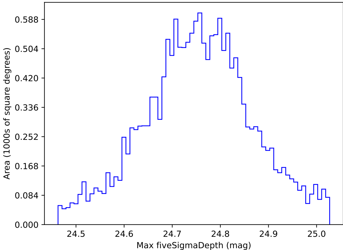
too_elab_r16_d3_griz_v3.4_10yrs WFD r band: Max fiveSigmaDepth
