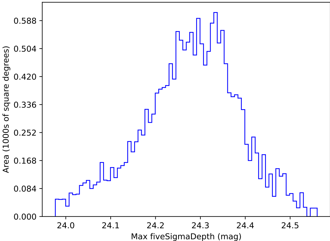
too_elab_r16_d3_griz_v3.4_10yrs WFD i band: Max fiveSigmaDepth
