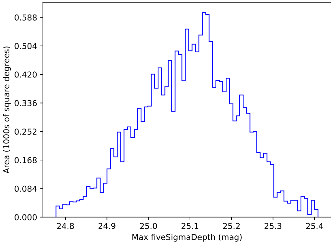
too_elab_r16_d3_griz_v3.4_10yrs WFD all bands: Max fiveSigmaDepth
