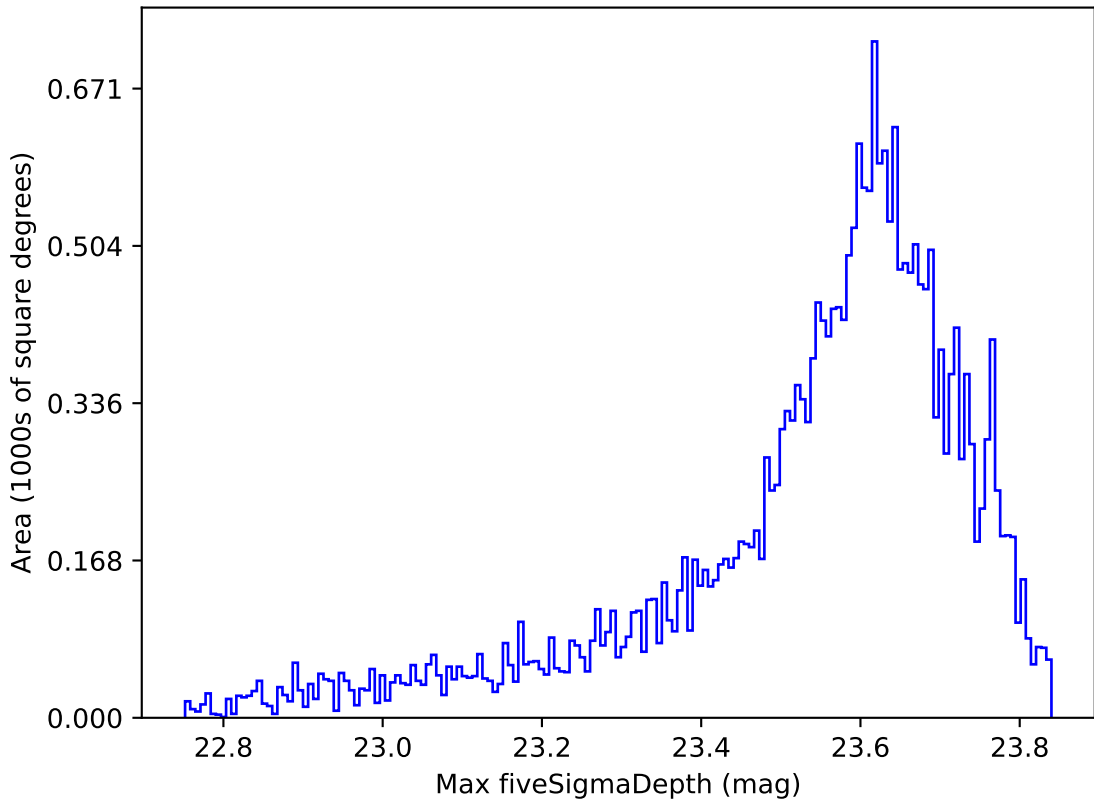
too_elab_r16_d3_griz_v3.4_10yrs All sky z band: Max fiveSigmaDepth
