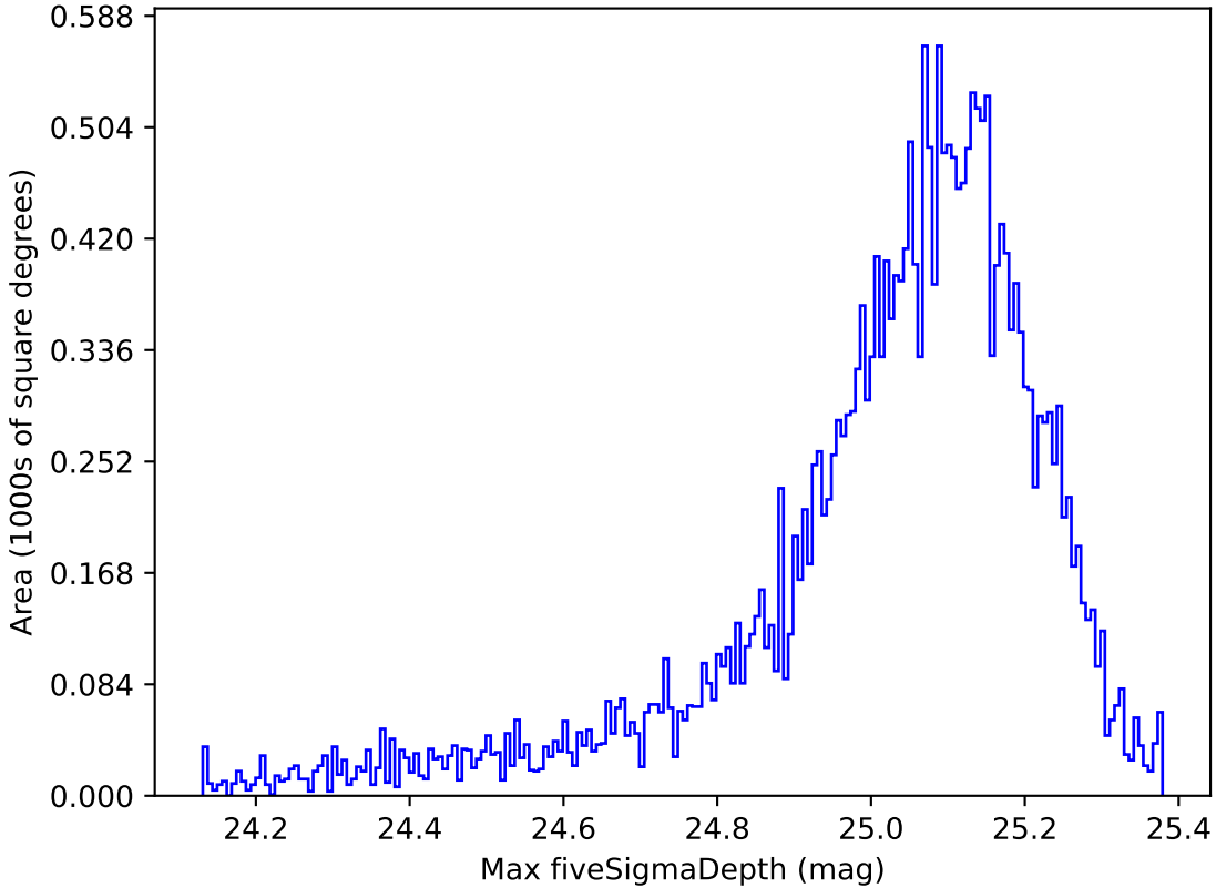
too_elab_r16_d3_griz_v3.4_10yrs All sky g band: Max fiveSigmaDepth
