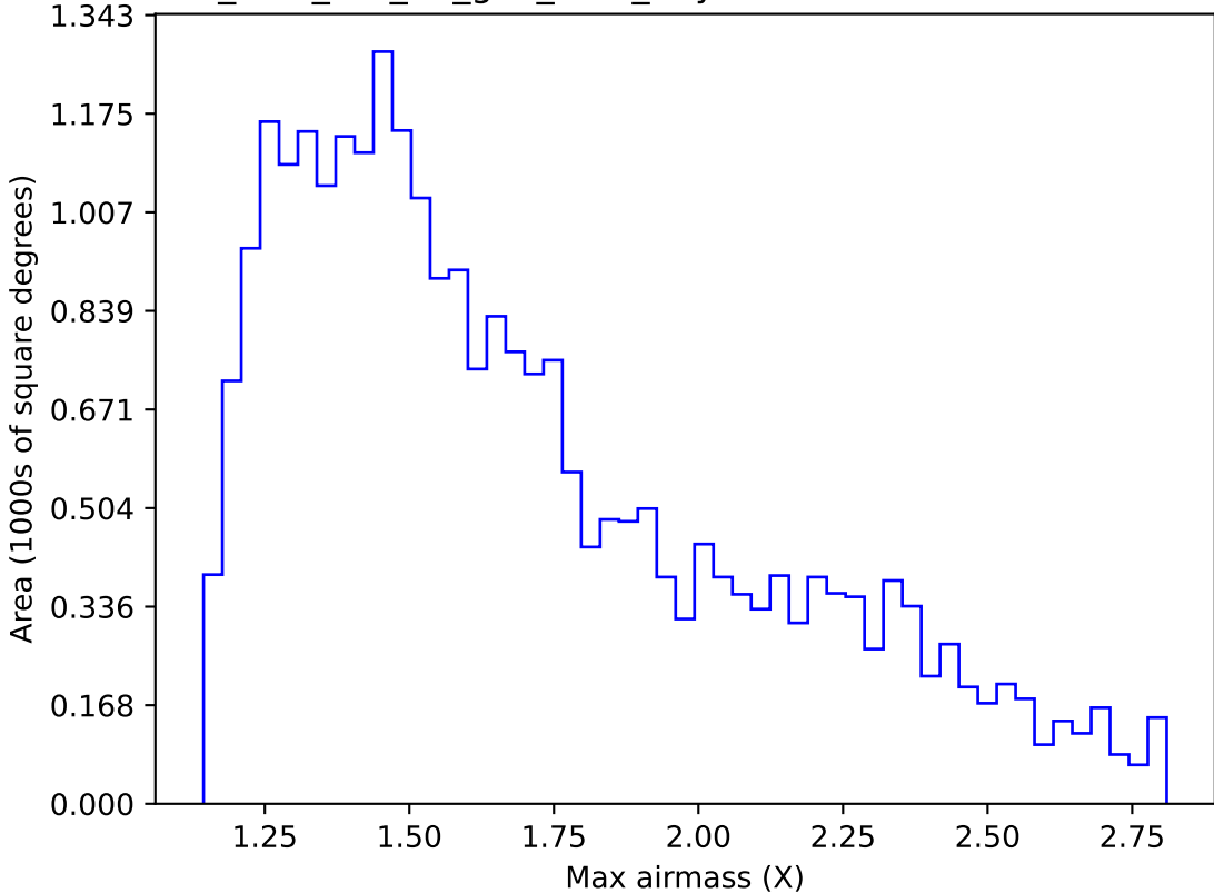
too_elab_r16_d3_griz_v3.4_10yrs Yr 1 z band: Max airmass
