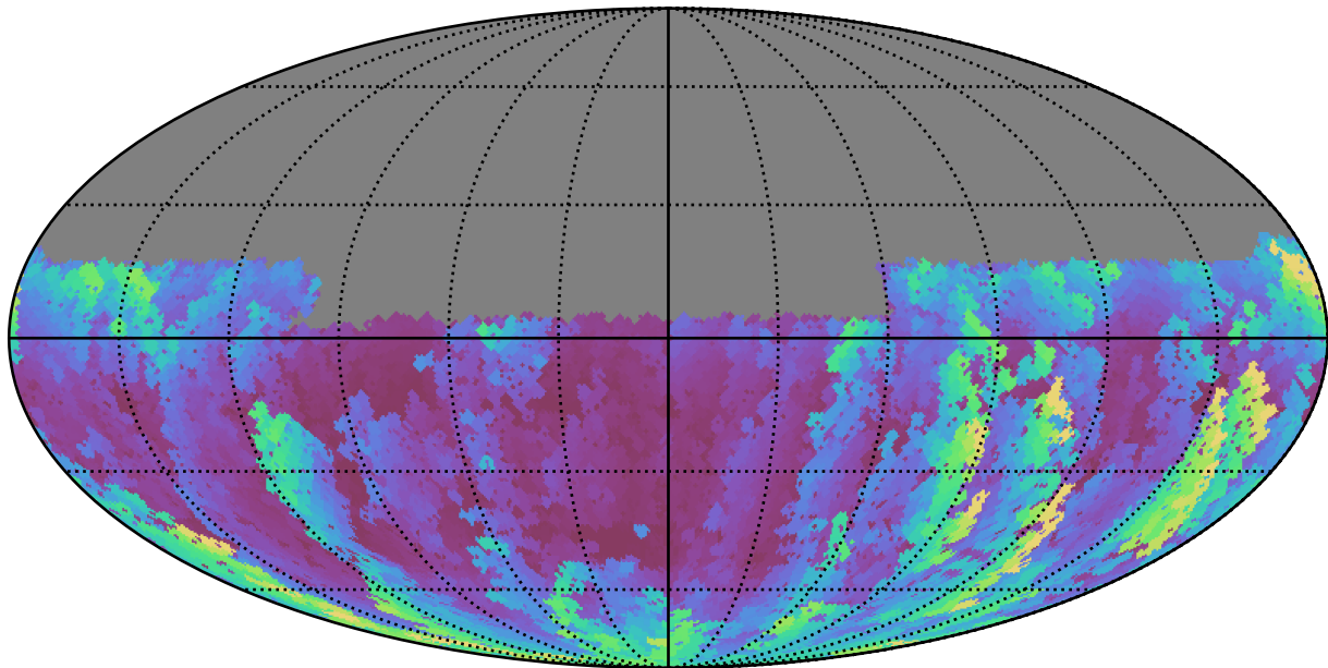
too_elab_r16_d3_griz_v3.4_10yrs Yr 1 u band: Max airmass
