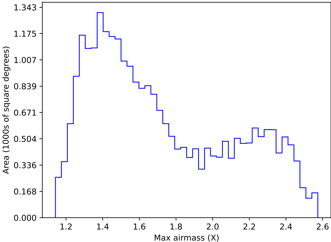
too_elab_r16_d3_griz_v3.4_10yrs Yr 1 r band: Max airmass
