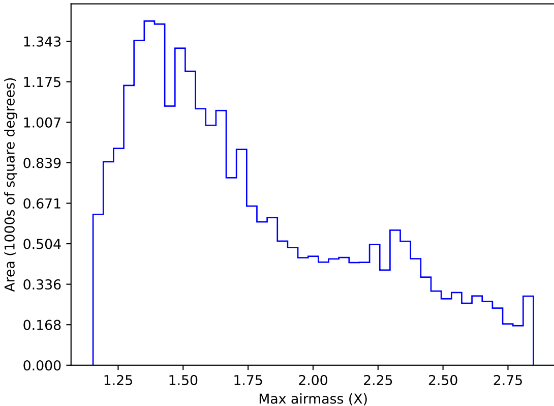
too_elab_r16_d3_griz_v3.4_10yrs Yr 1 i band: Max airmass
