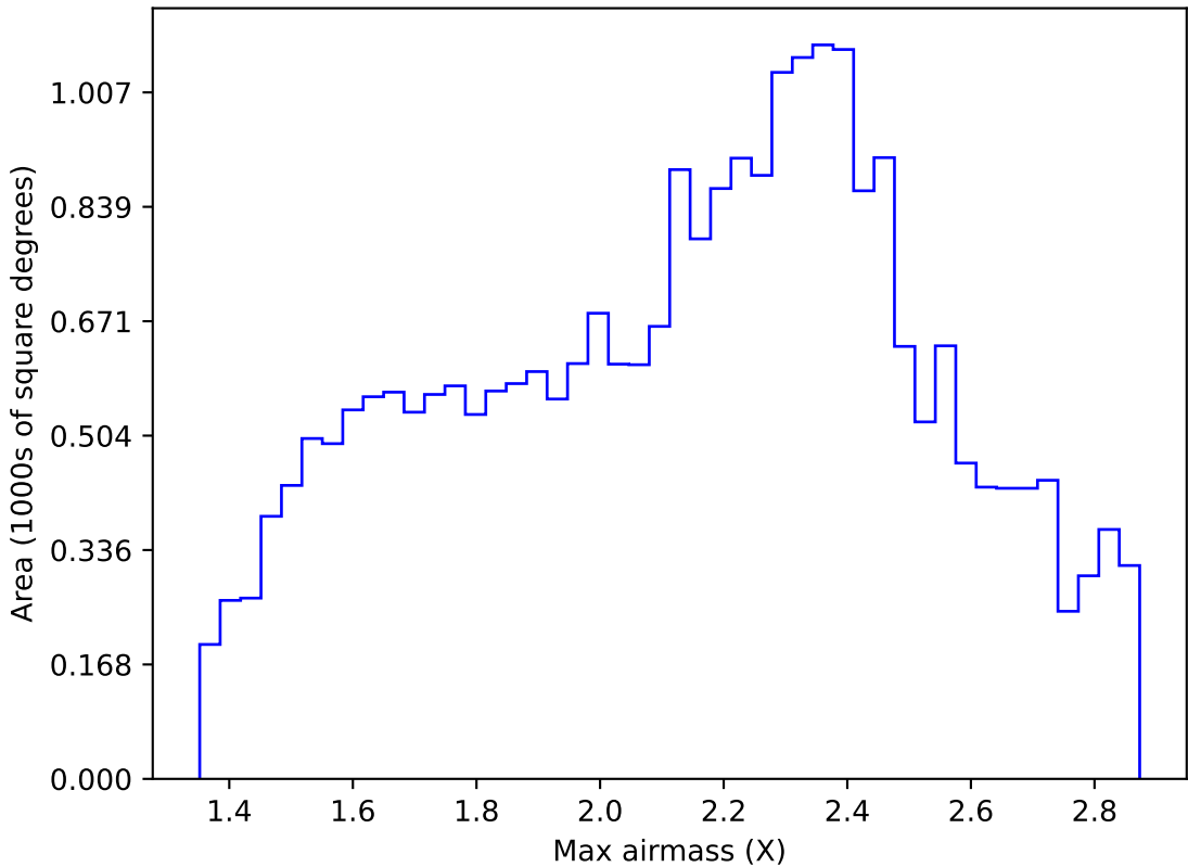
too_elab_r16_d3_griz_v3.4_10yrs Yr 1 all bands: Max airmass
