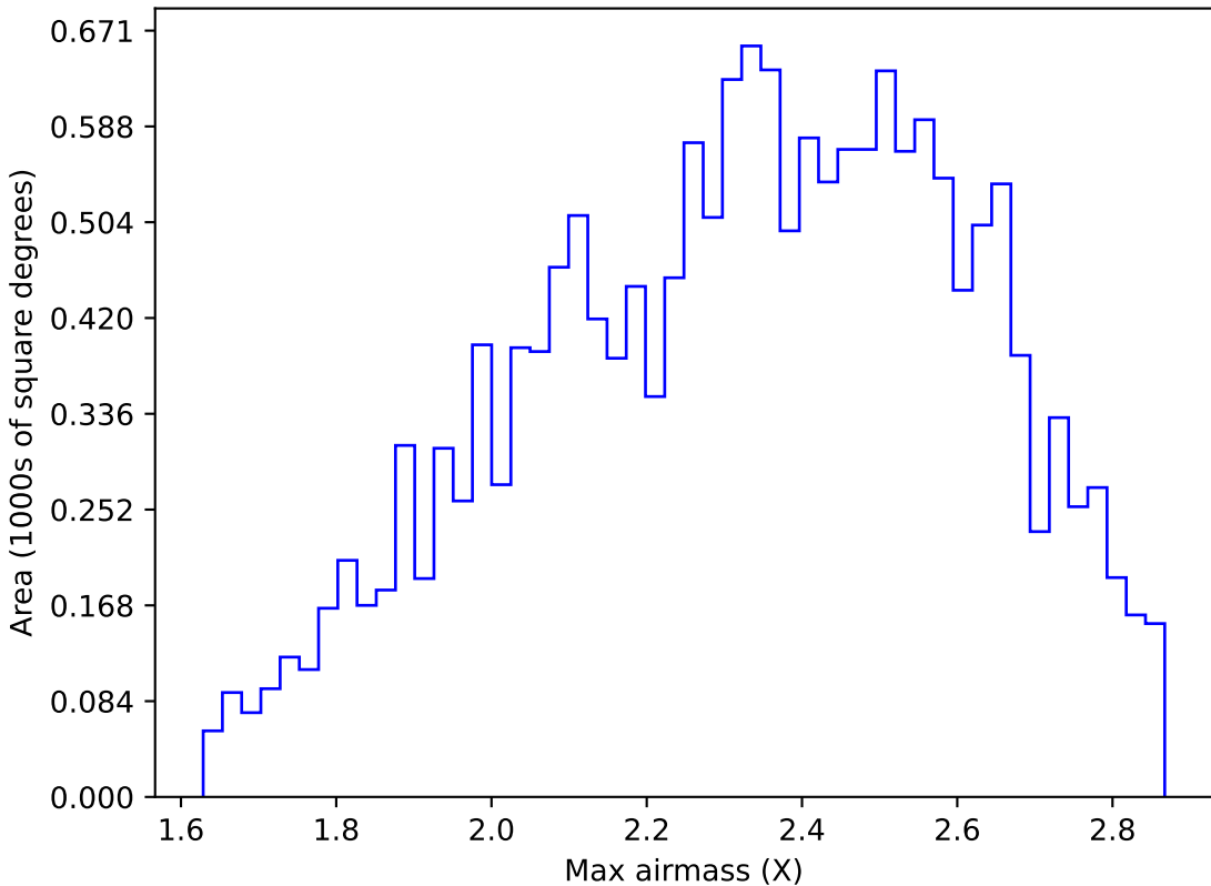
too_elab_r16_d3_griz_v3.4_10yrs WFD y band: Max airmass
