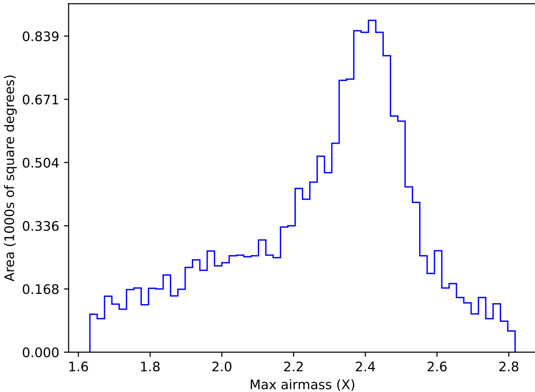
too_elab_r16_d3_griz_v3.4_10yrs WFD r band: Max airmass
