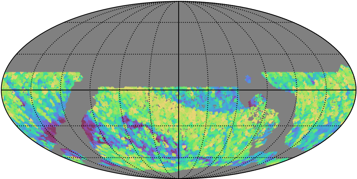
too_elab_r16_d3_griz_v3.4_10yrs WFD all bands: Max airmass
